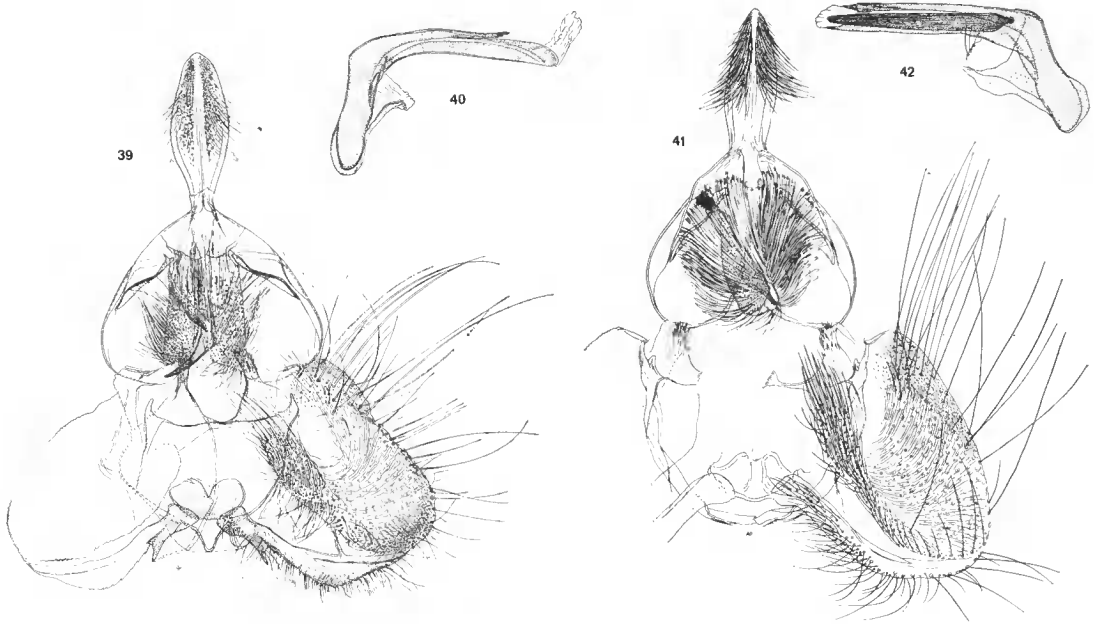
FIG. 39-42. — Male genitalia of Madagascan Tortricinae. 39, Goniotorna (Tenuisaccula) trignoma sp. nov., holotype ; 40, the same, aedeagus ; 41, G. (T.) chondrocentra sp. nov., holotype ; 42, the same, aedeagus.
